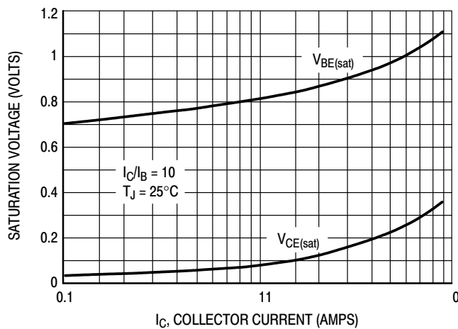
Figure 8. 4H11 On-Voltages
