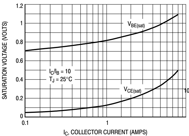
Figure 9. 5H11 On-Voltages
