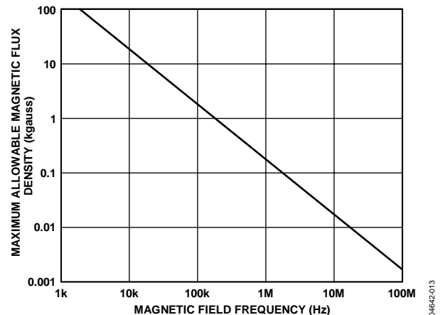
Figure 13. Maximum Allowable External Magnetic Flux Density
